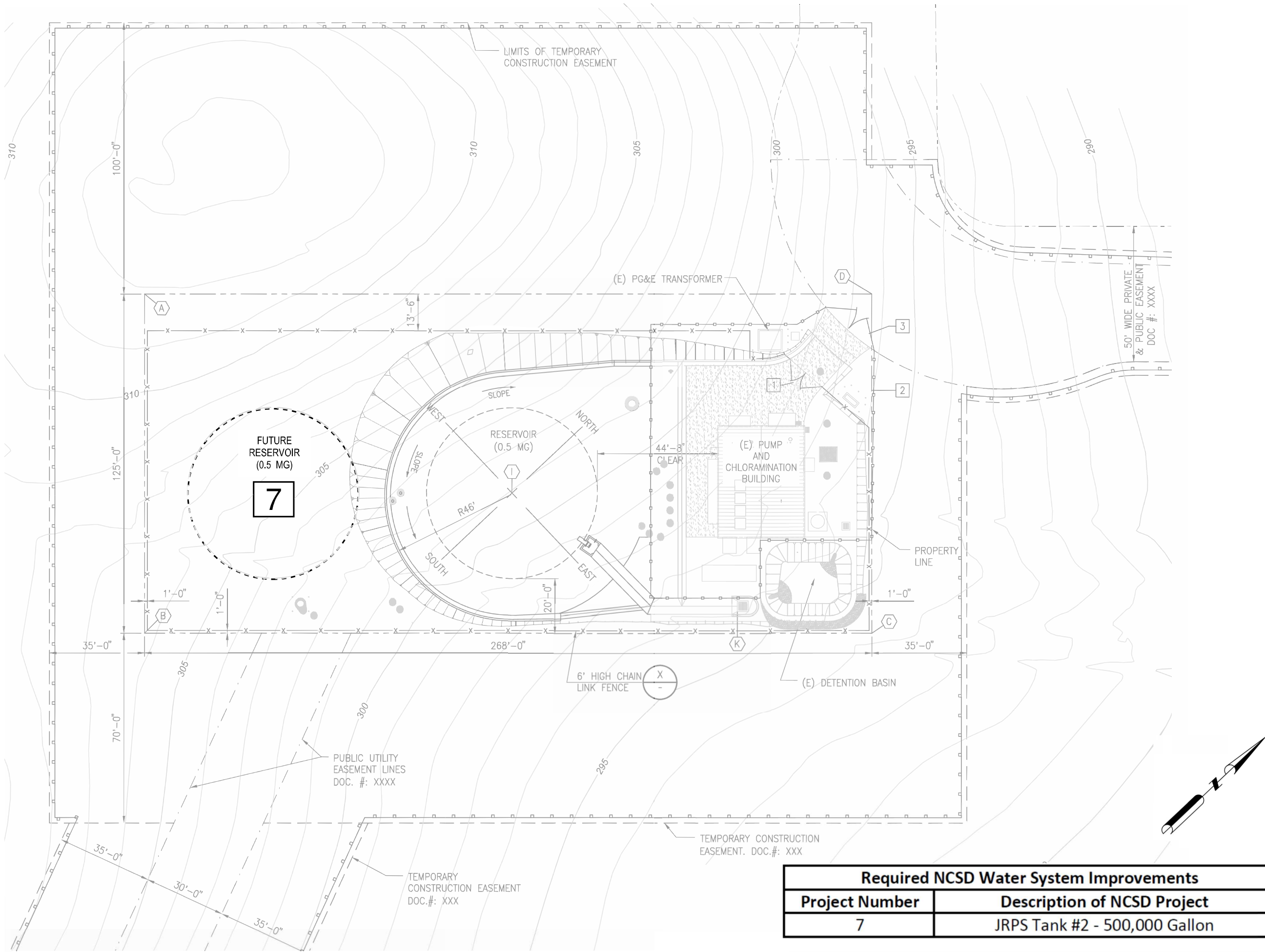
Figure 6-2 Proposed Joshua Road Pump Station Reservoir Improvements
