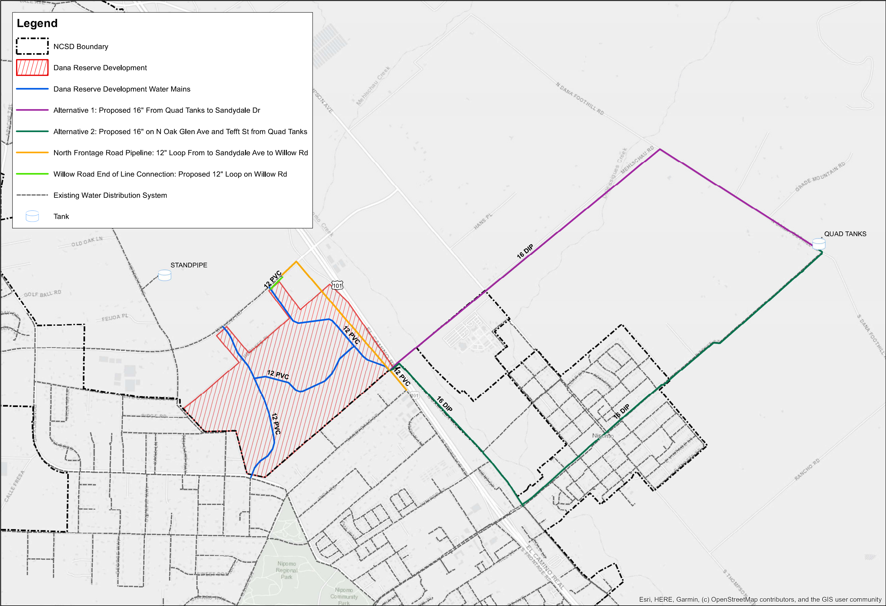
Figure 2-1 Proposed Pipeline Improvements for District Water System
