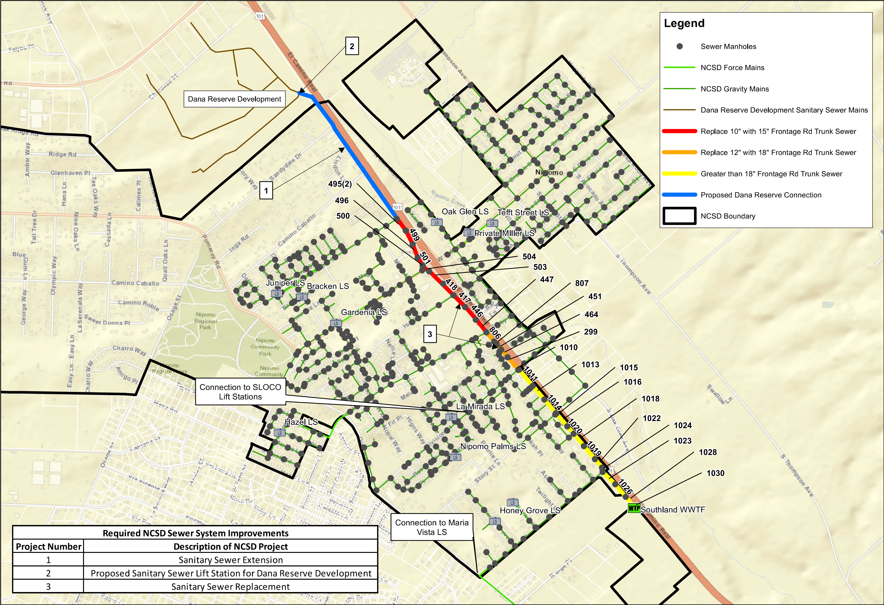
Figure 3-2 Wastewater Collection System Improvements
