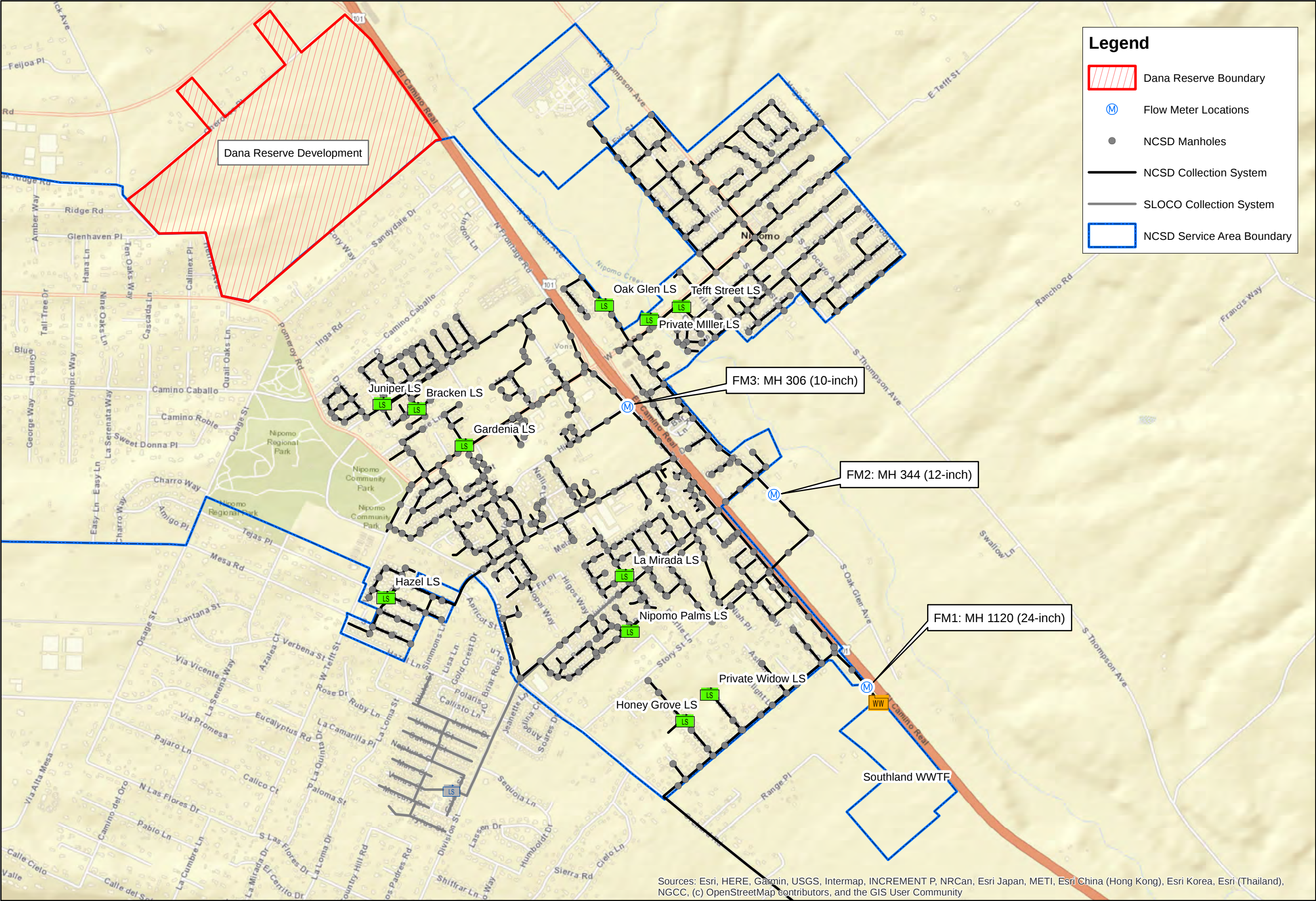
Figure 3-1: Flow Meter Locations
