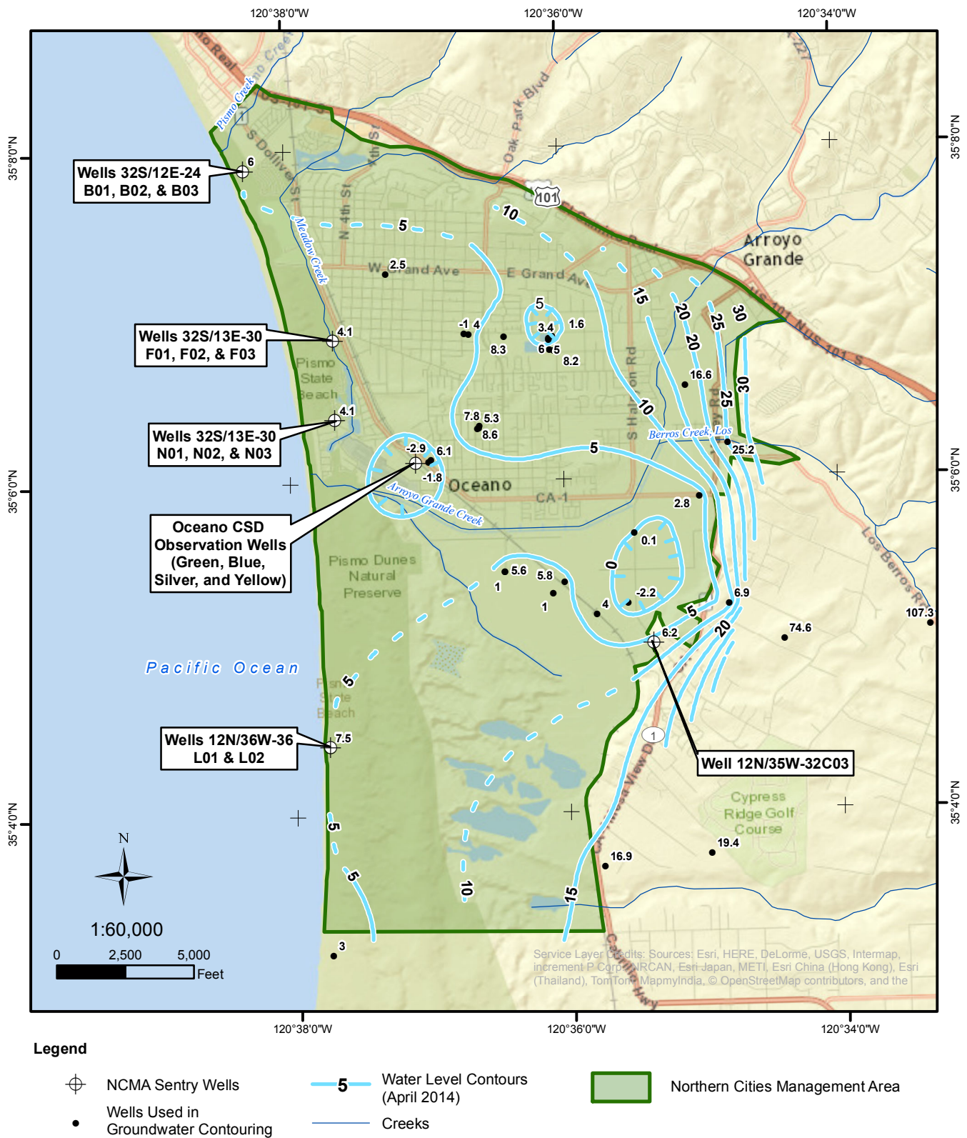
WATER LEVEL CONTOURS, APRIL 2014 Northern Cities Management Area San Luis Obispo County, California
