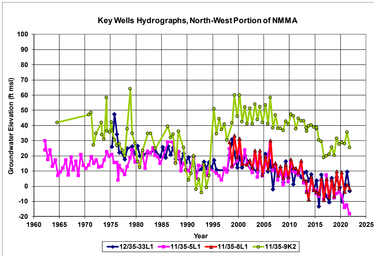
Figure 6-2. Key Wells Hydrographs, North-West Portion of NMMA
