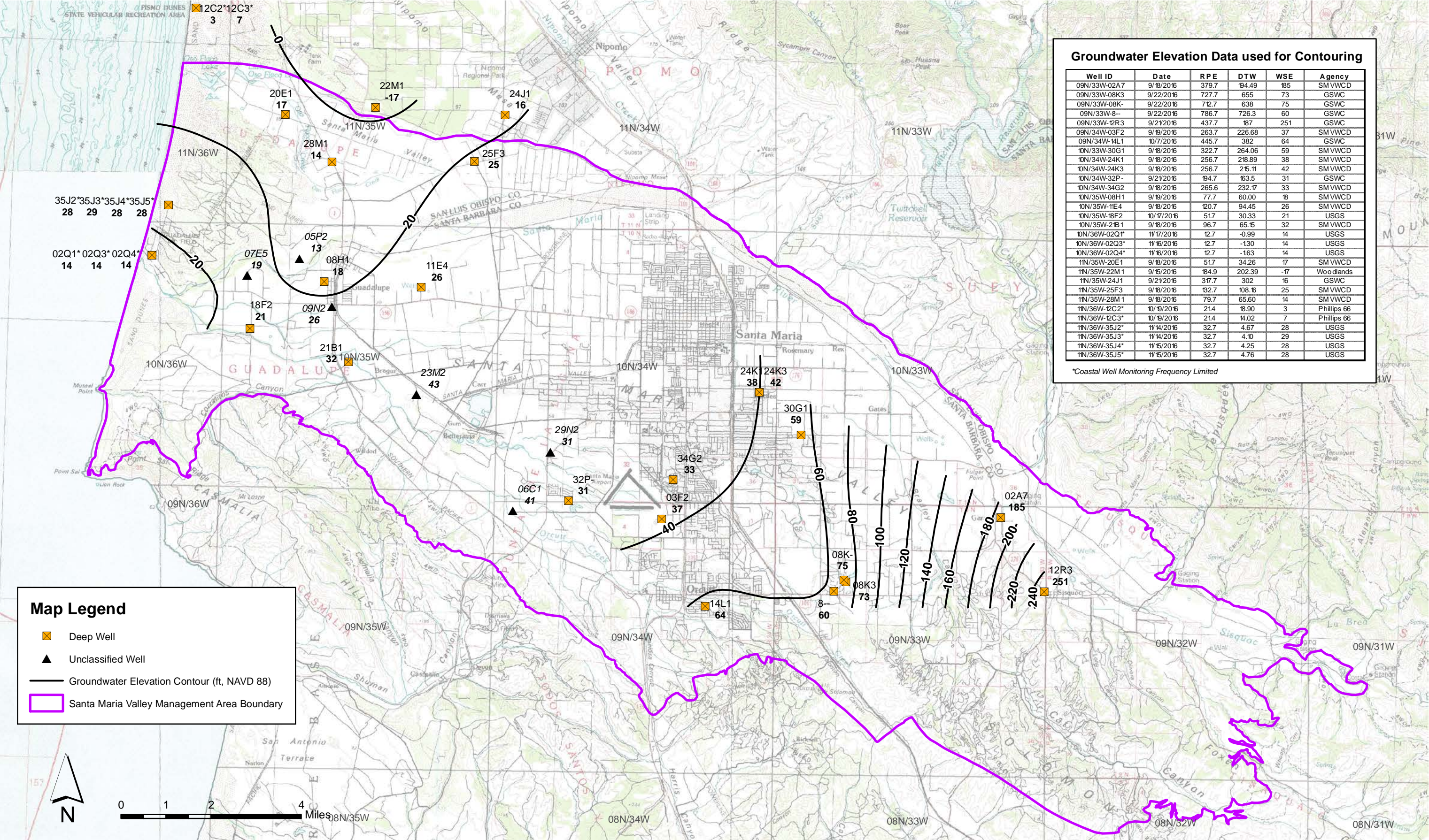
Figure 2.1-3d Contours of Equal Groundwater Elevation, Deep Zone, Fall (September 15 - October 17) 2016 Santa Maria Valley Management Area
