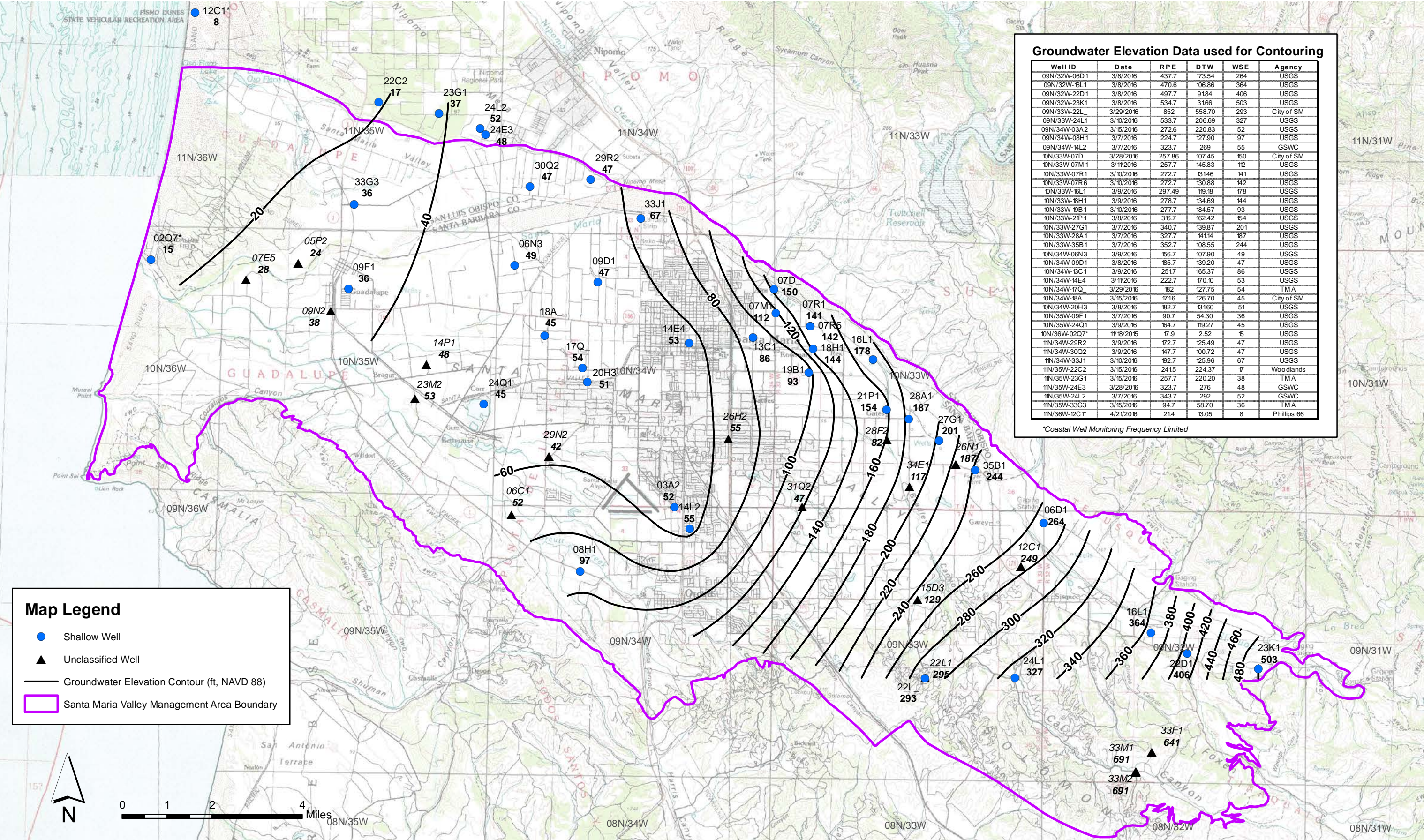
Figure 2.1-3a Contours of Equal Groundwater Elevation, Shallow Zone, Spring (March 7-29) 2016 Santa Maria Valley Management Area
