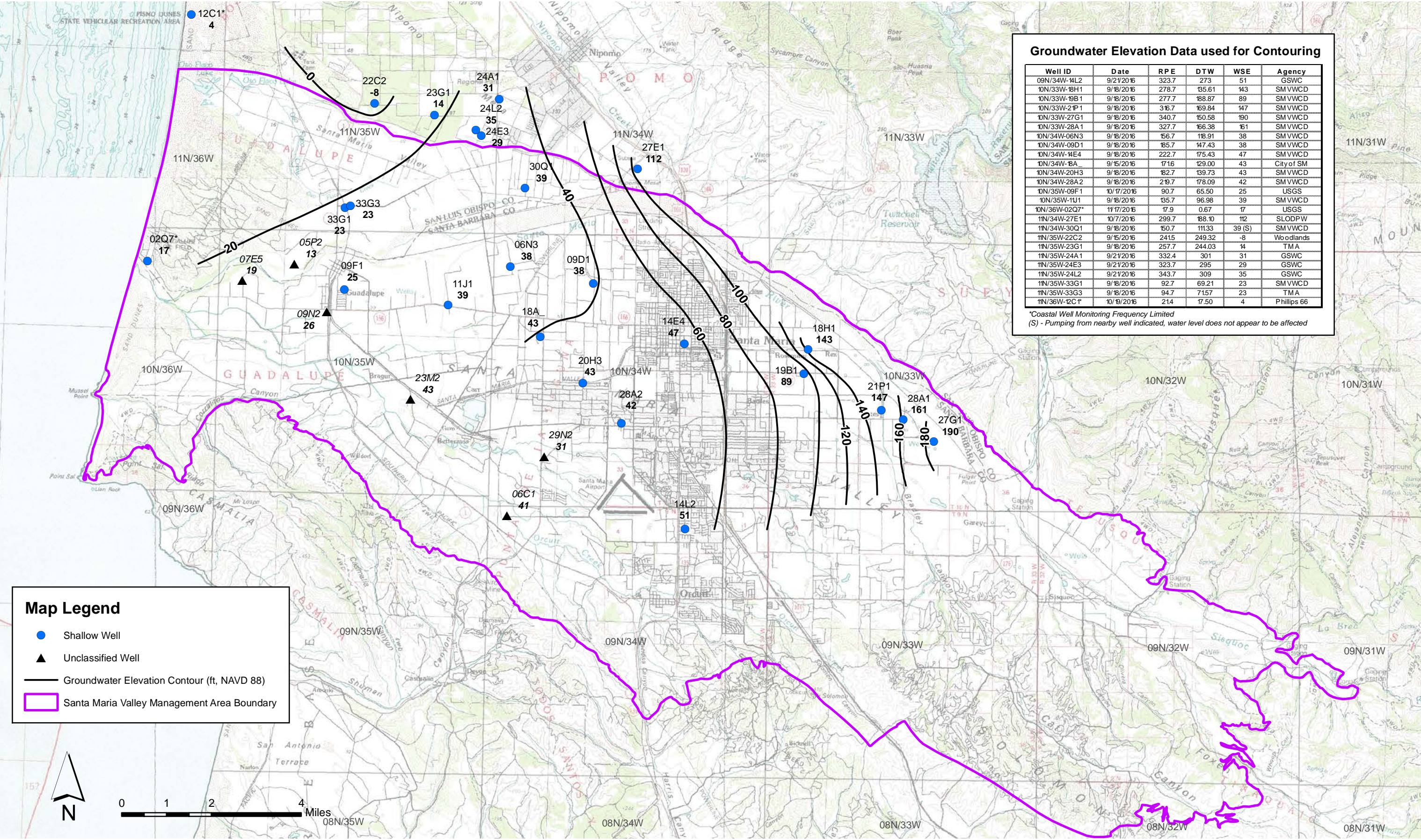
Figure 2.1-3b Contours of Equal Groundwater Elevation, Shallow Zone, Fall (September 15 - October 17) 2016 Santa Maria Valley Management Area
