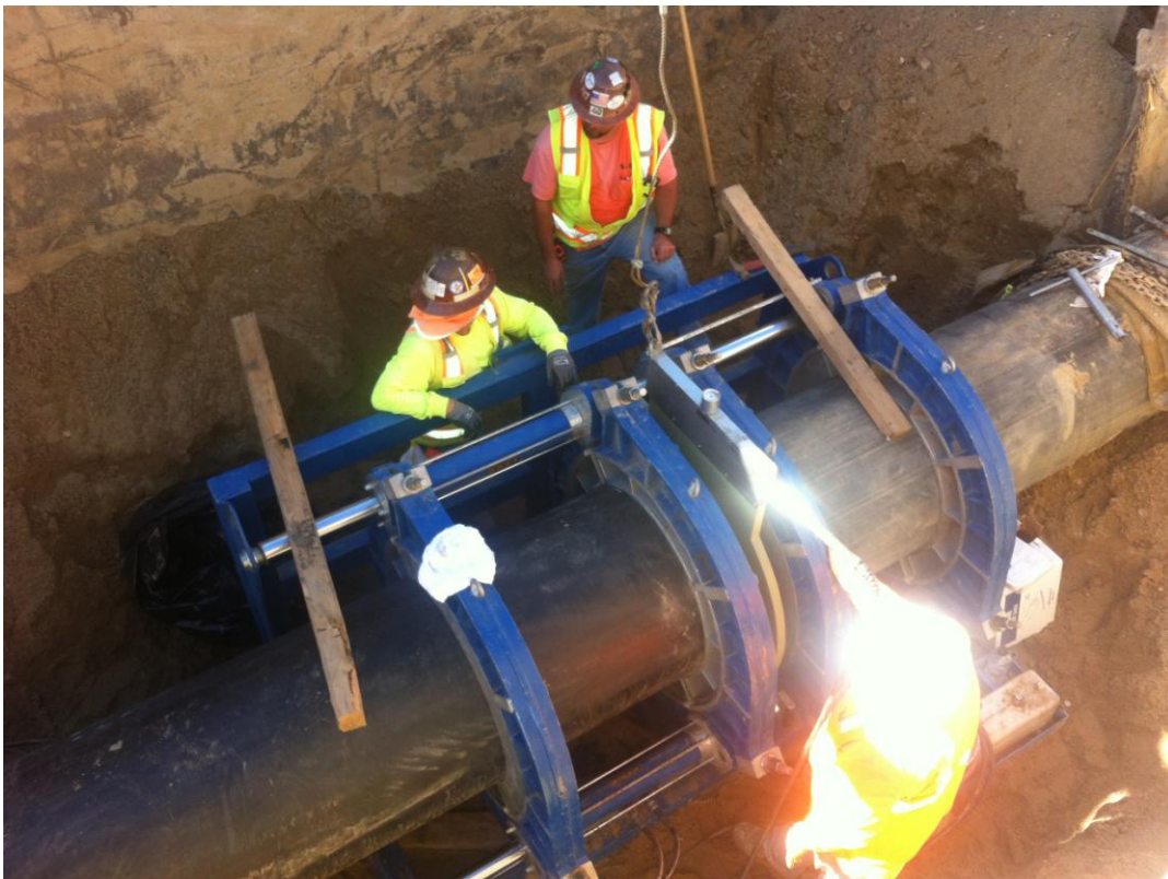
Pipe fusing machine in place with heater plate between HDPE pipe ends (reaches 472 degrees F).
