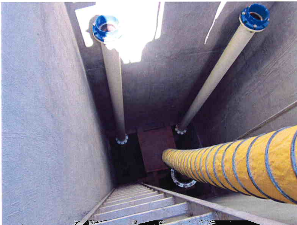
Cushman installing RAS/WAS Piping inside RAS/WAS Pump Station #2.
