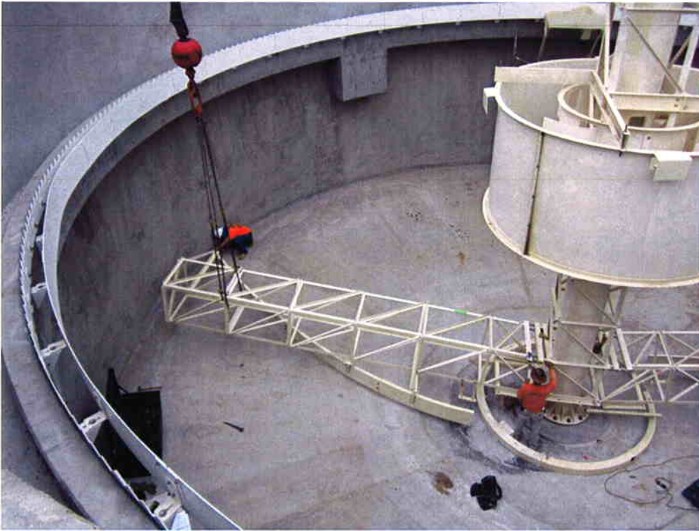
Installing mechanisms installed inside Clarifier #1.
