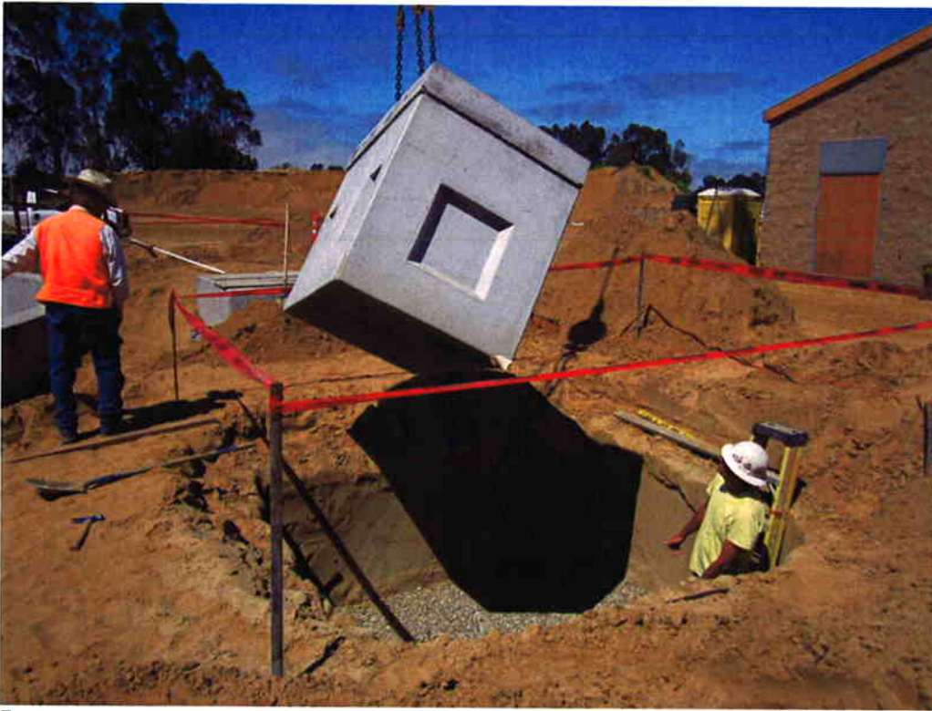
Bergelectric and Cushman installing Pull Box #25.
