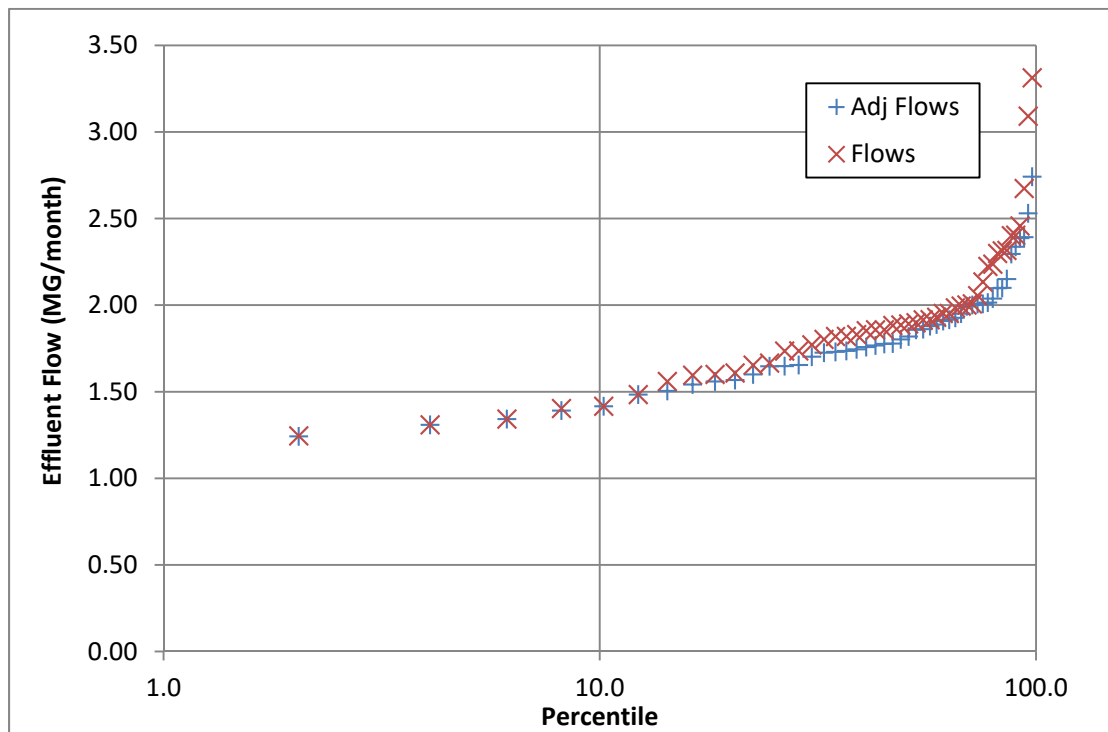
Figure 2-4: Arithmetic Probability Plot of Monthly Effluent Flows
