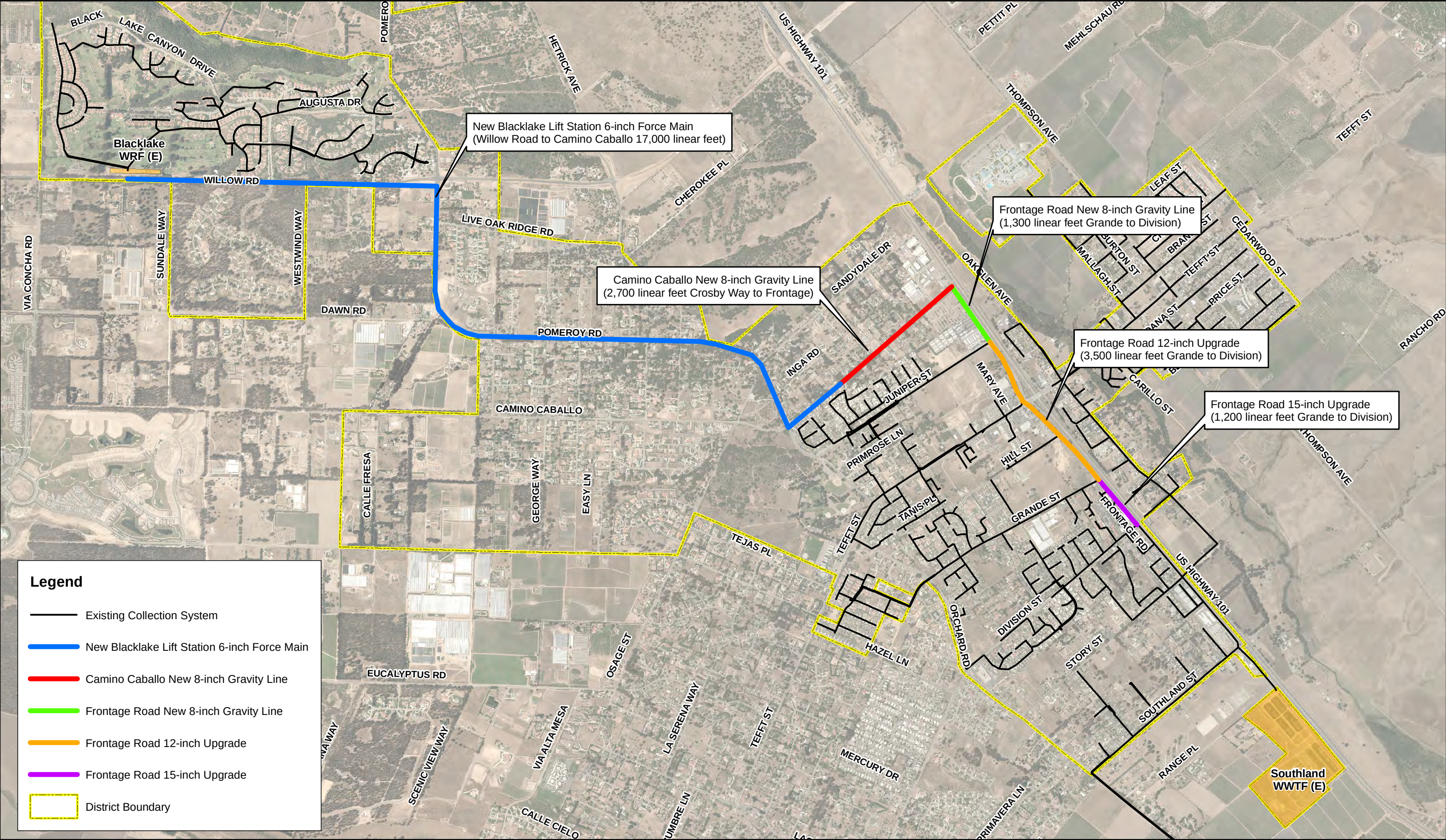
NIPOMO COMMUNITY SERVICES DISTRICT BLACKLAKE SEWER MASTER PLAN FIGURE 8-1: REGIONALIZATION PIPELINE IMPROVEMENTS
