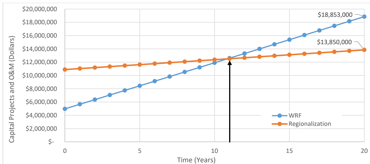
Figure ES-1: Comparative 20-year Life Cycle Costs for WRF Operation and Regionalization
