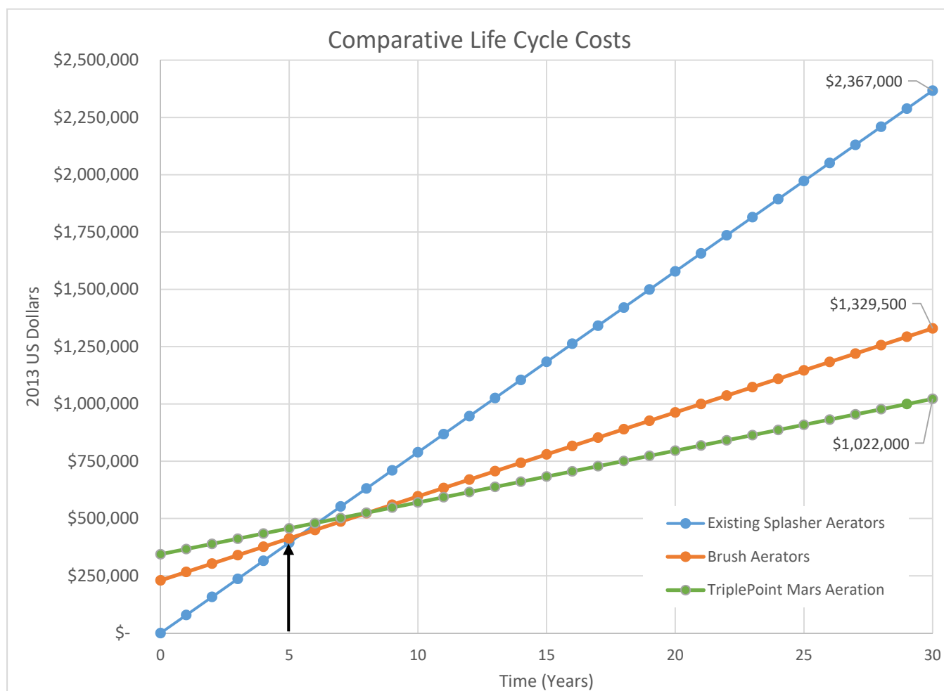
Figure 5-2: Comparative 30-year Life Cycle Costs for Splasher, Brush, and Diffused Aeration Systems
