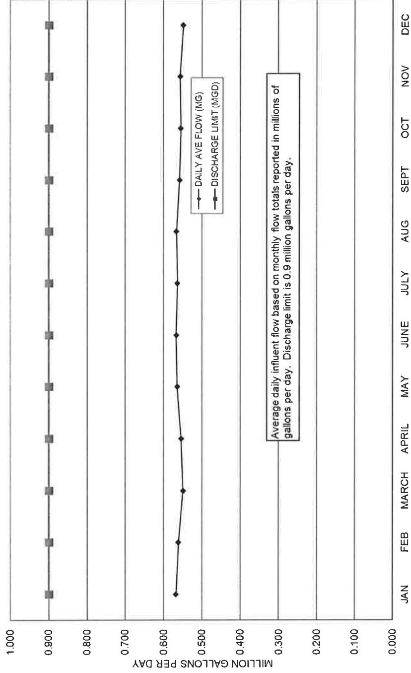
Southland Wastewater Treatment Facility 2017 Monthly Averages Influent Flow - Million Gallons Per Day (MGD)
