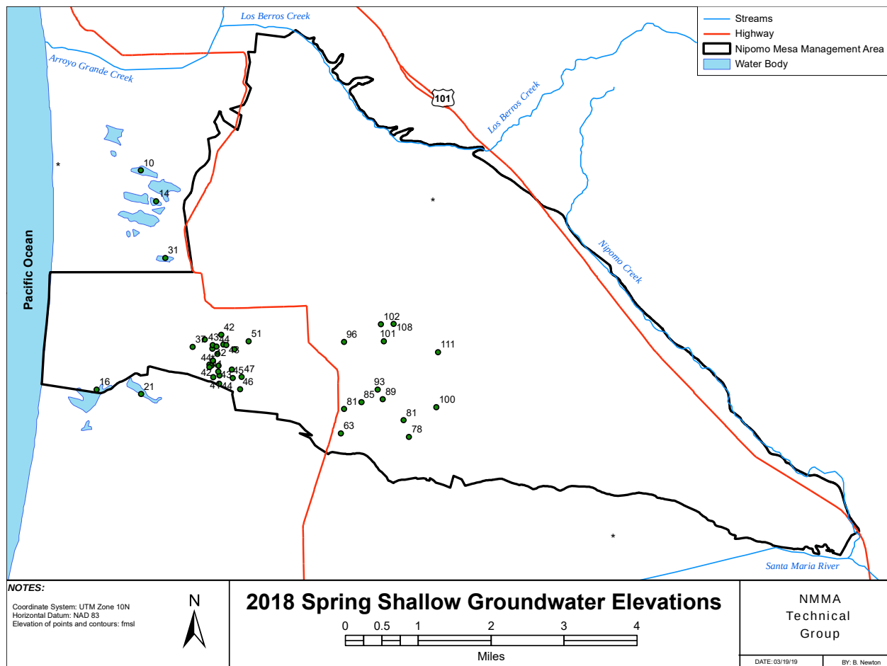
Figure 3-1: 2018 Spring Shallow Dune Sand Aquifer Groundwater Elevations
