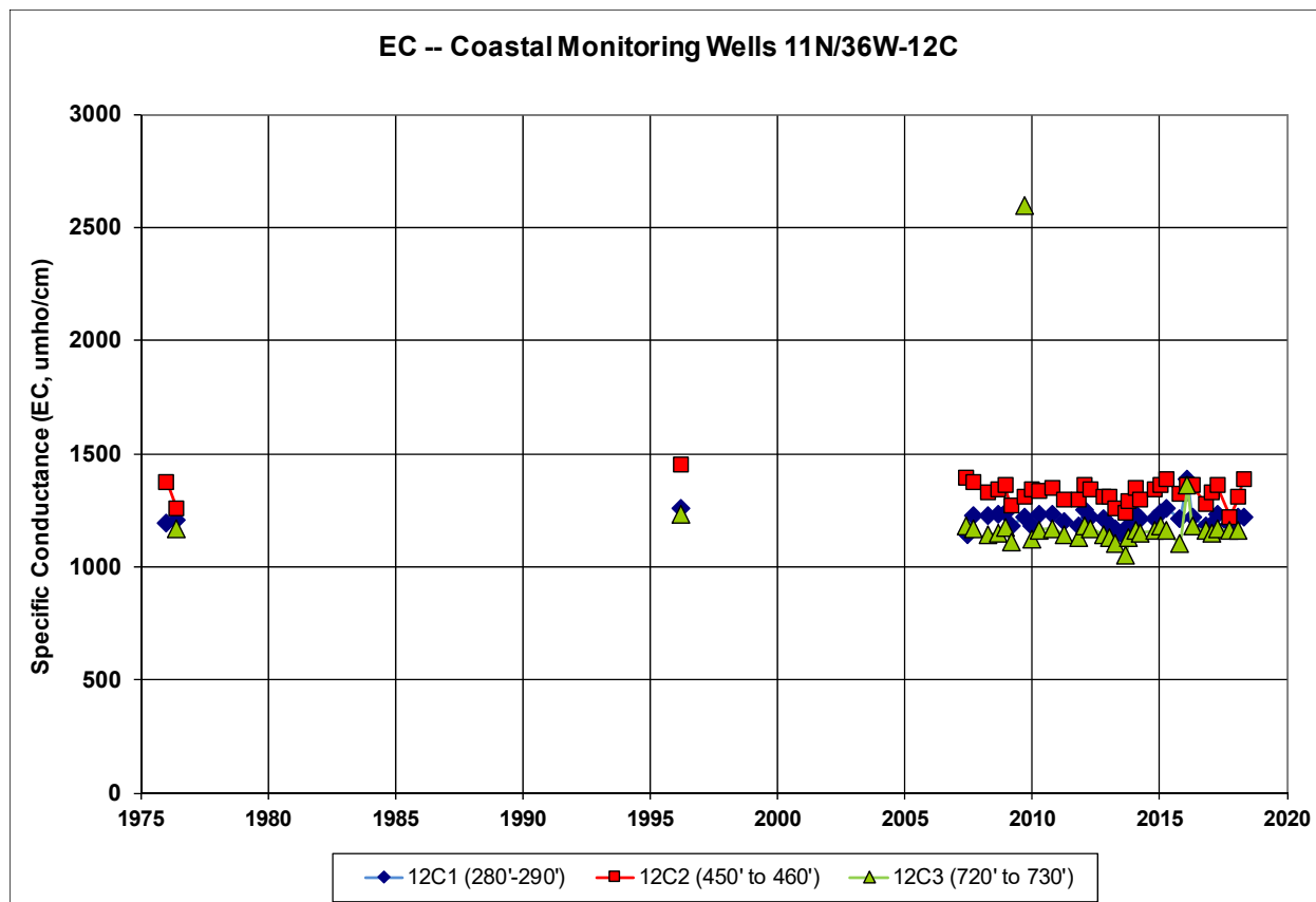
Figure 6-10. Electrical Conductivity in Coastal Well 11N/36W-12C
