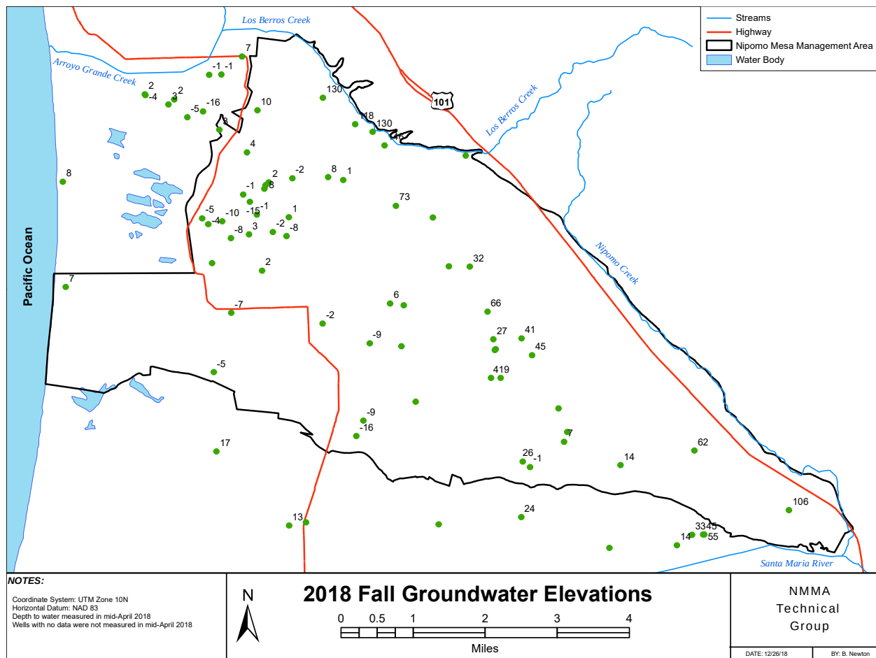
Figure 3-4. 2018 Fall Deep Aquifer Groundwater Elevations
