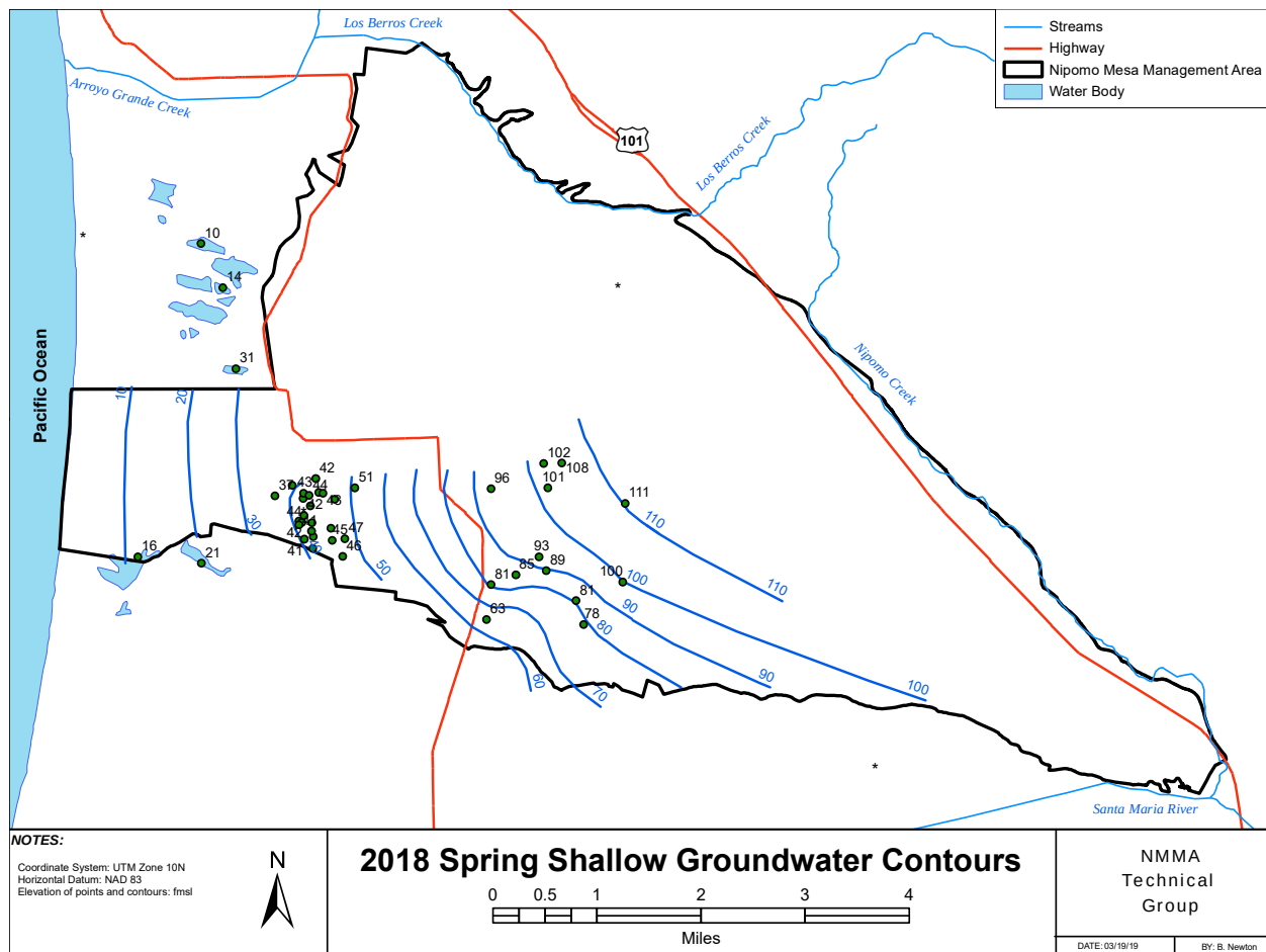
Figure 6-5. 2018 Spring Shallow Dune Sand Aquifer Groundwater Contours
