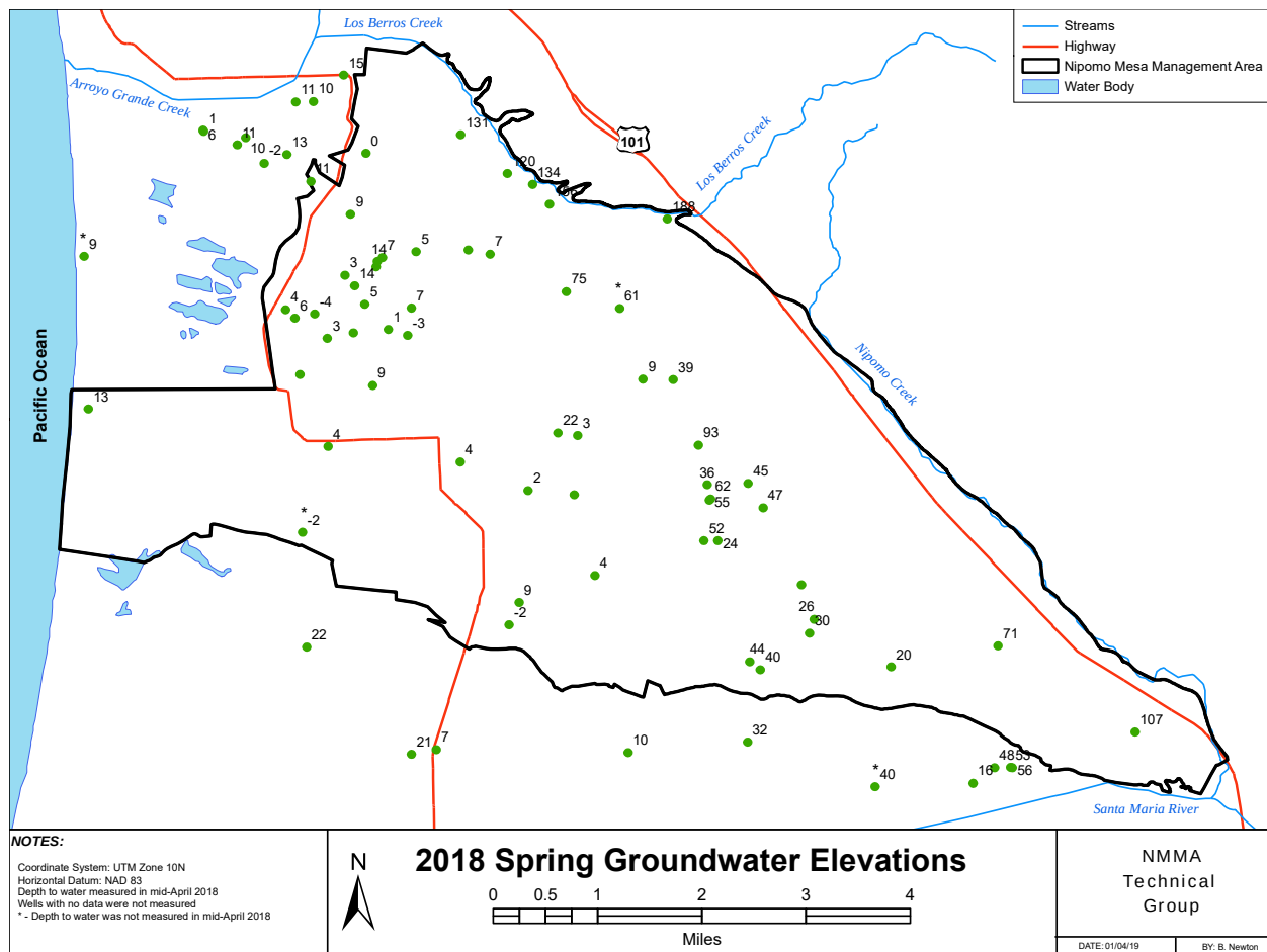
Figure 3-2. 2018 Spring Deep Aquifer Groundwater Elevations
