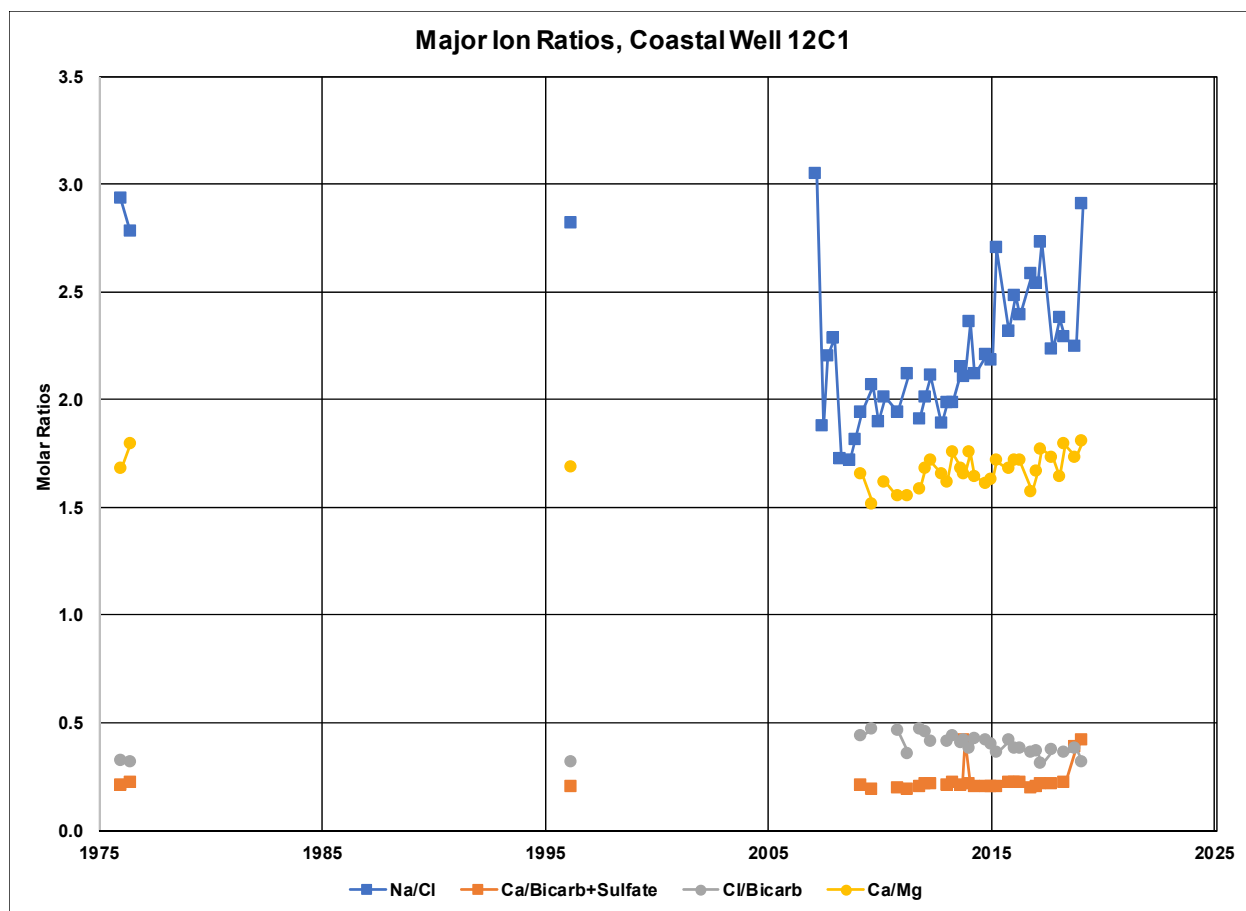
Figure 6-16. Major Ion Ratio for Coastal Well 12C1
