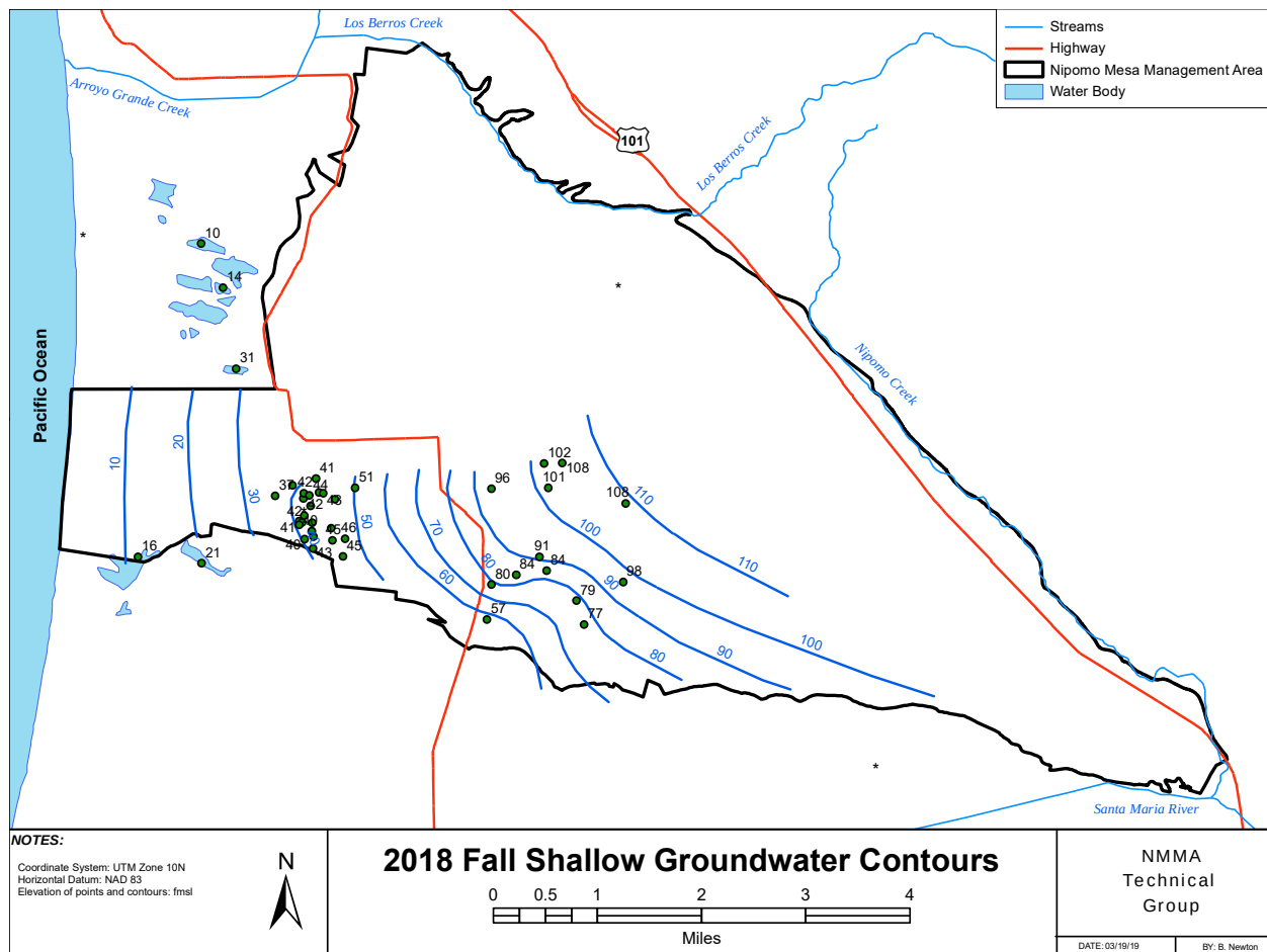
Figure 6-7. 2018 Fall Shallow Sand Dune Aquifer Groundwater Contours
