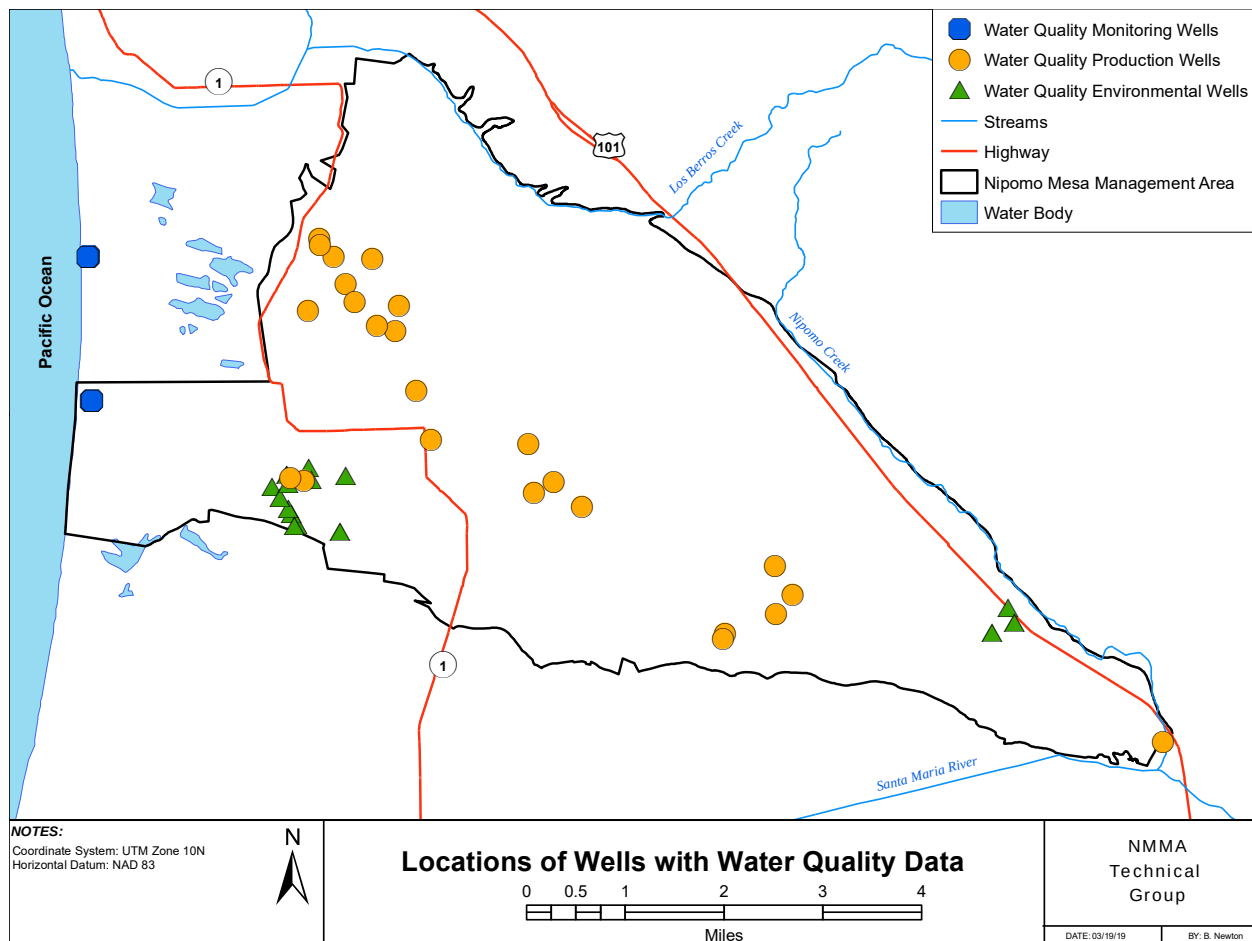
Figure 3-5. 2018 Locations of wells with water quality data
