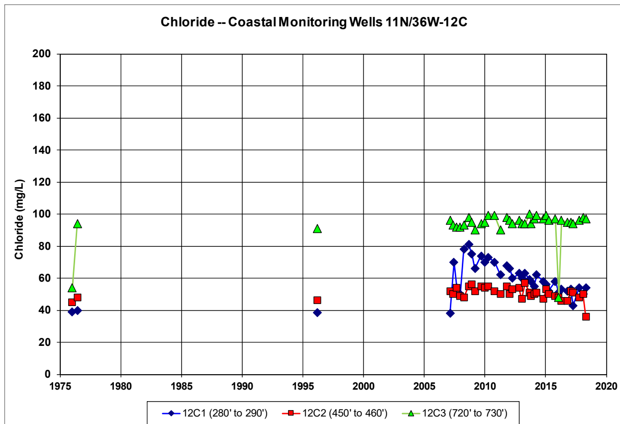
Figure 6-9. Chloride in Coastal Well 11N/36W-12C
