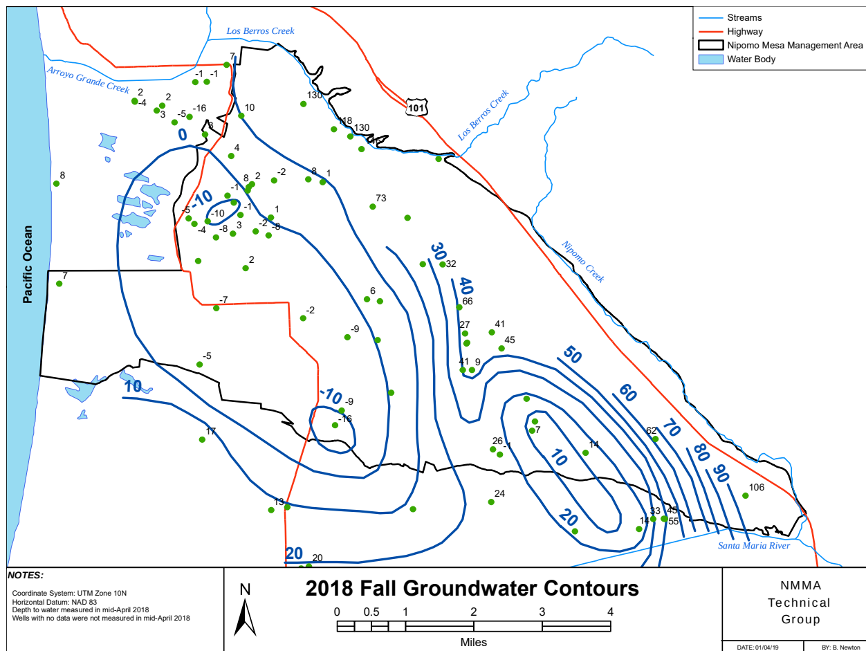
Figure 6-8. 2018 Fall Deep Aquifer Groundwater Contours
