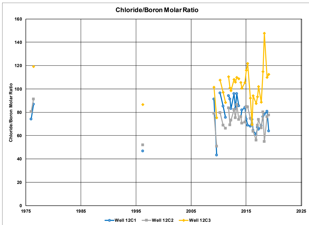
Figure 6-19. Chloride/Boron Ratio for Coastal Wells
