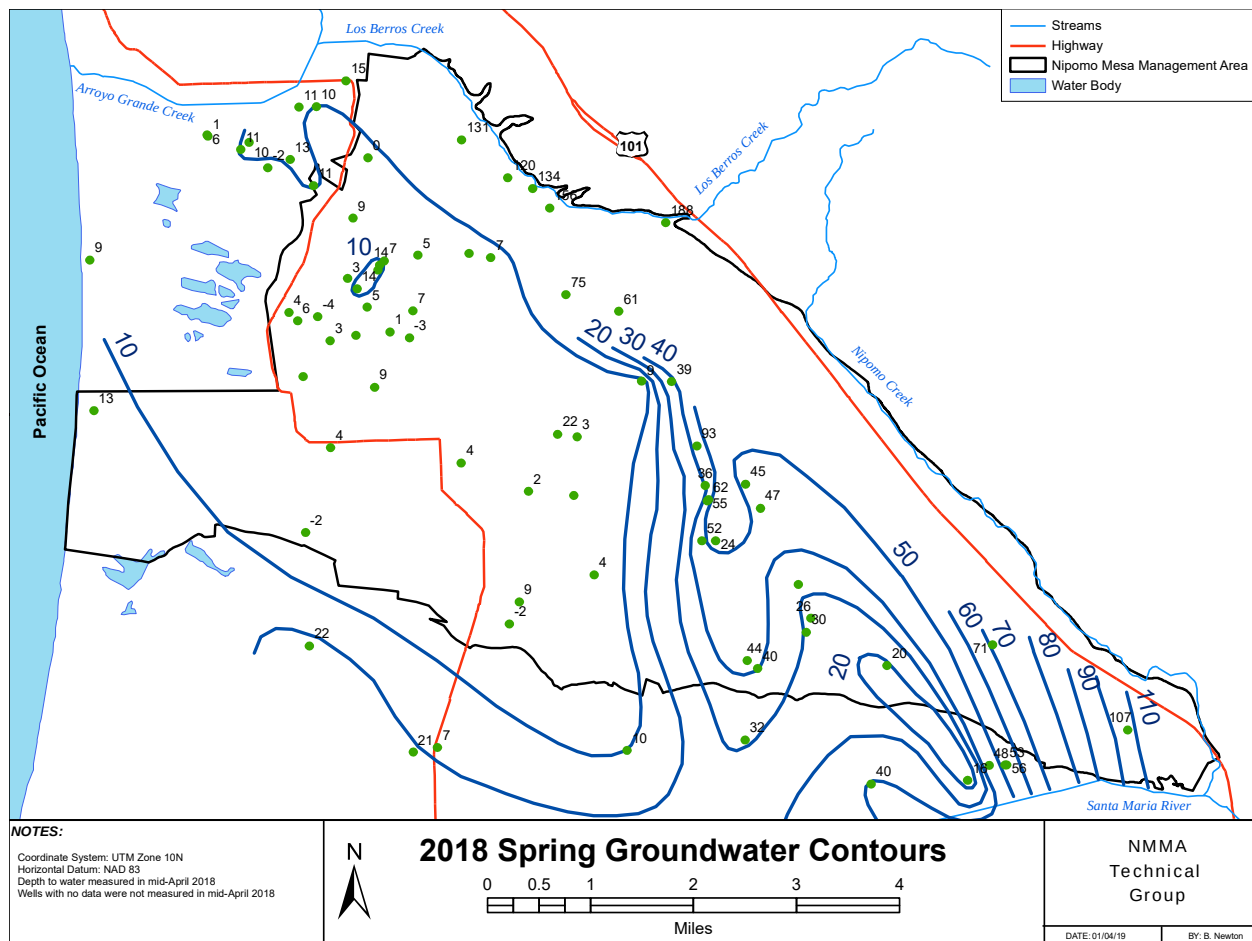
Figure 6-6. 2018 Spring Deep Aquifer Groundwater Contours
