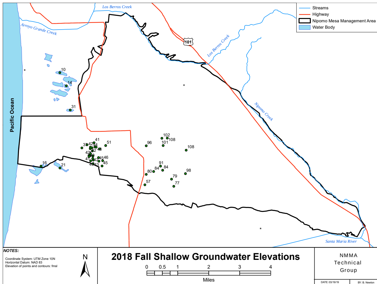
Figure 3-3: 2018 Fall Shallow Dune Sand Aquifer Groundwater Elevations
