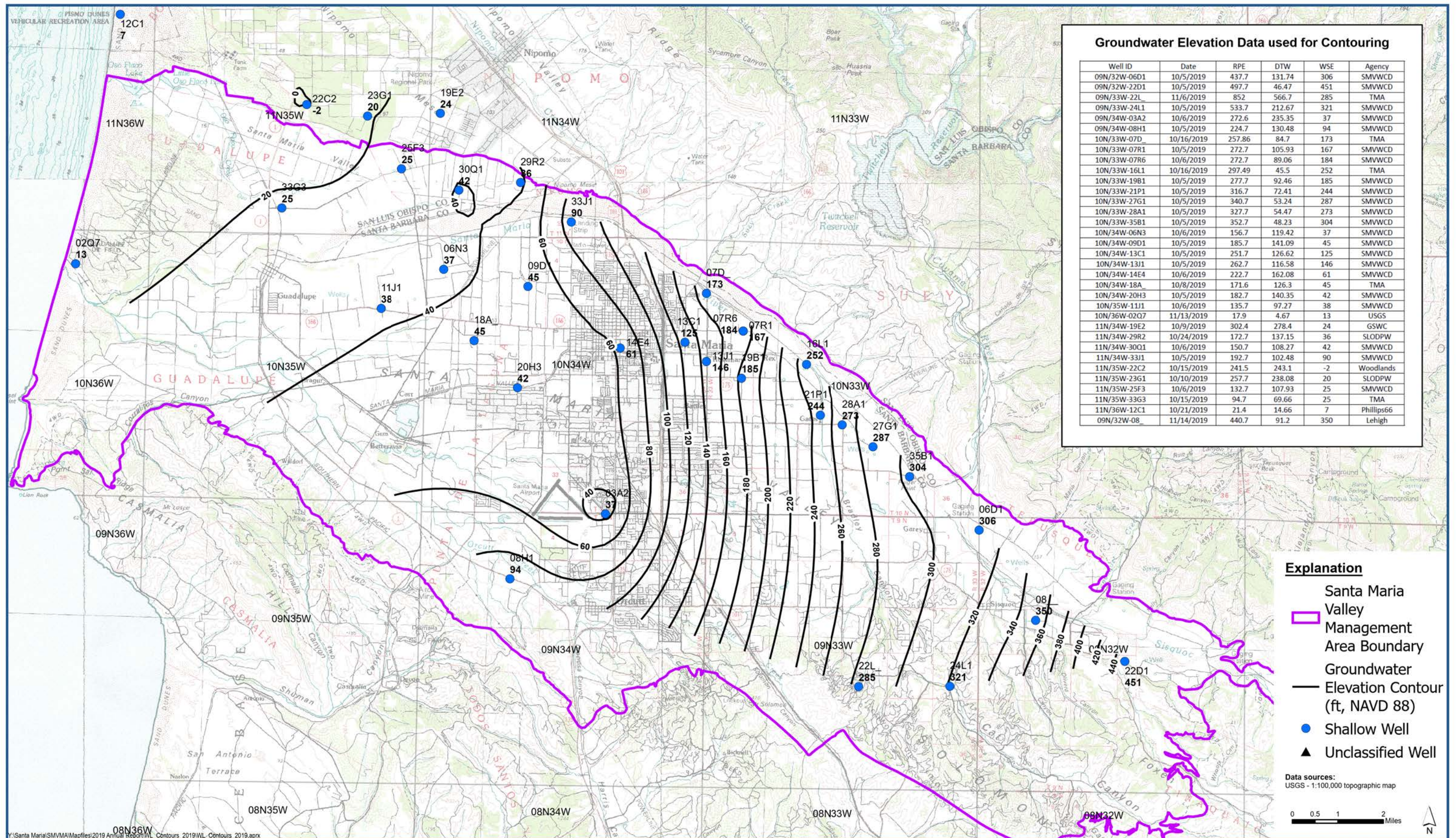
Contours of Equal Groundwater Elevation, Shallow Zone, Fall (October 5 - November 14) 2019 Santa Maria Valley Management Area
