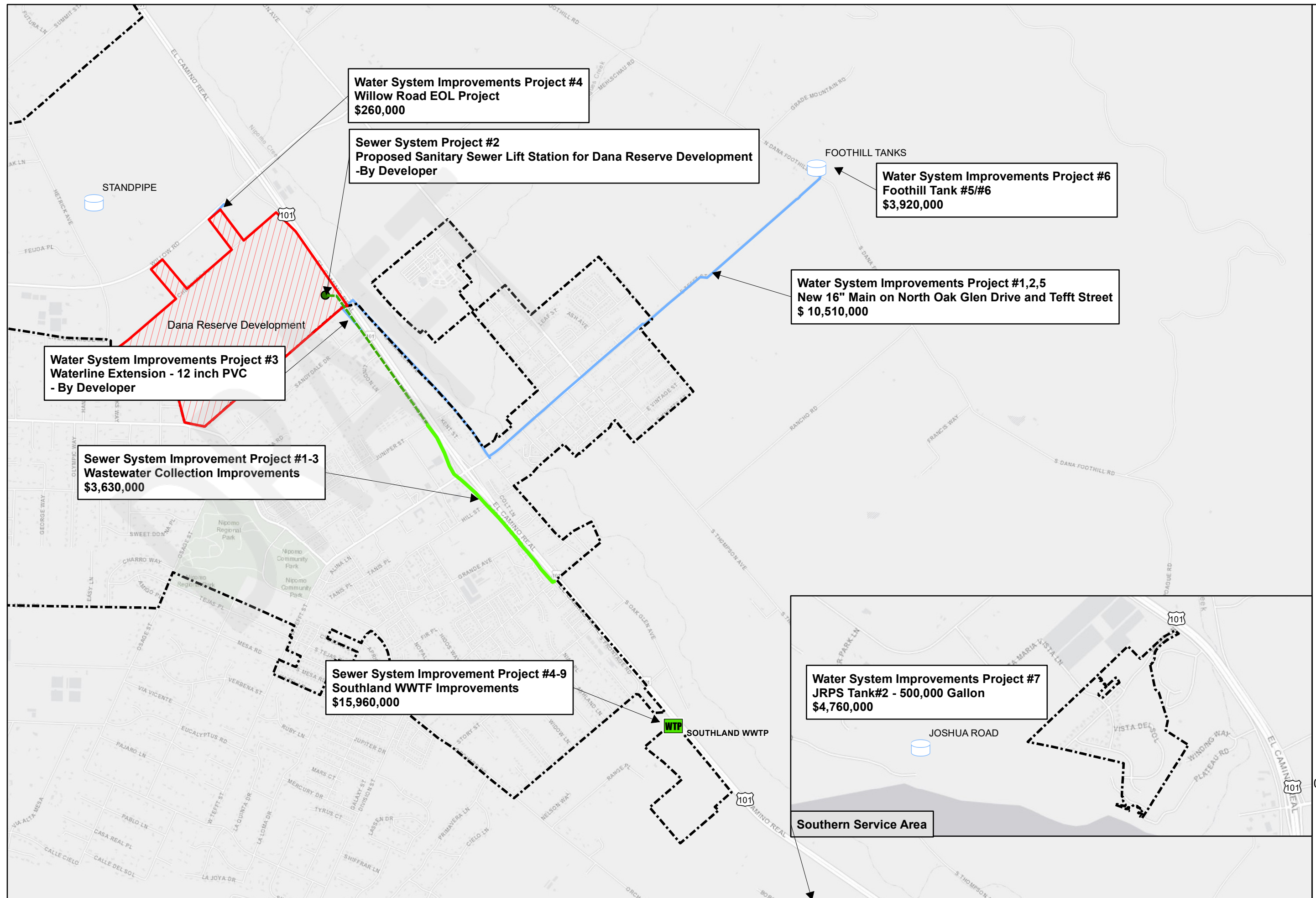
Figure 6-5 Proposed Water and Sewer System Improvements
