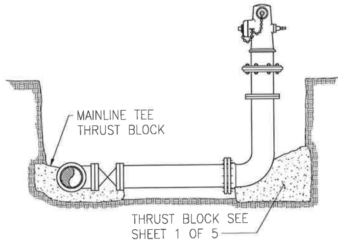
FIRE HYDRANT
