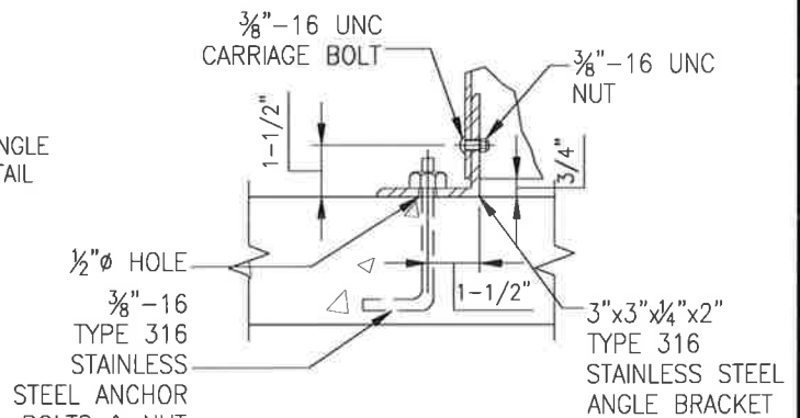
BOLTDOWN DETAIL
