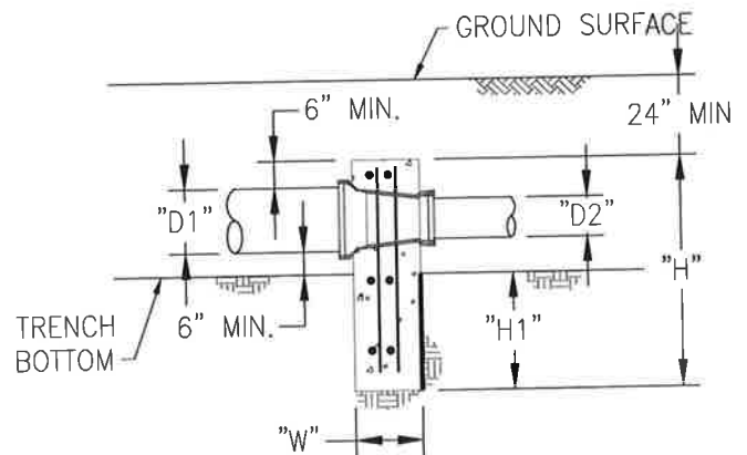
SECTION
