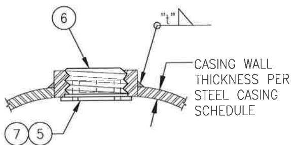
GROUT FITTING DETAIL
