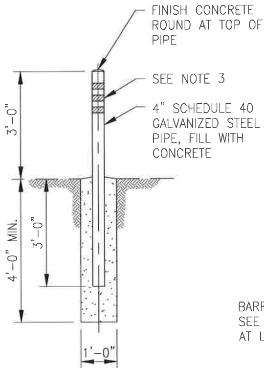
BOLLARD/BARRICADE DETAIL
