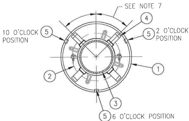
CROSS-SECTION
