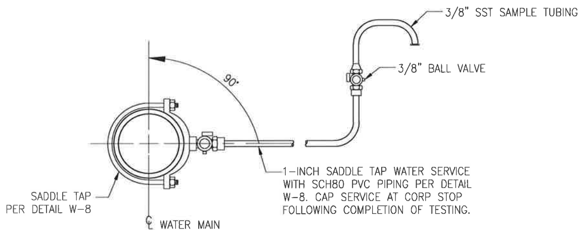
TEMPORARY WATER QUALITY SAMPLING PORT DETAIL
