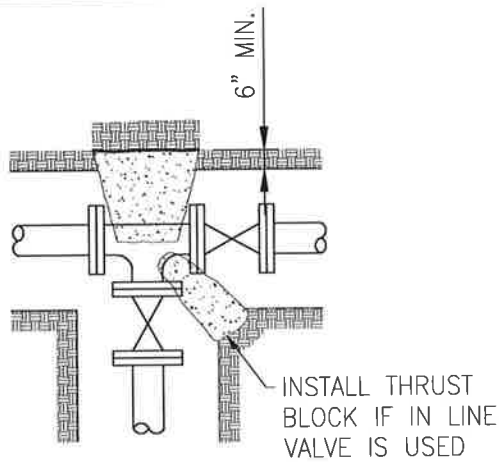
OUTLET OR FIRE HYDRANT
