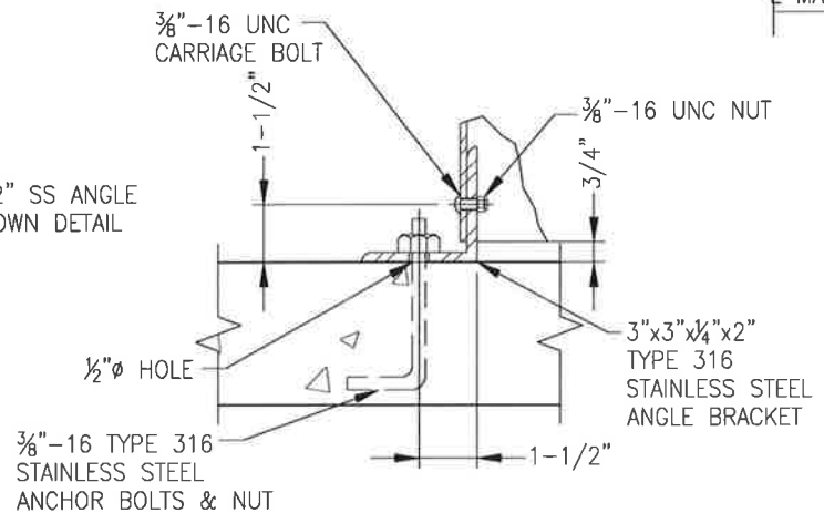
BOLTDOWN DETAIL
