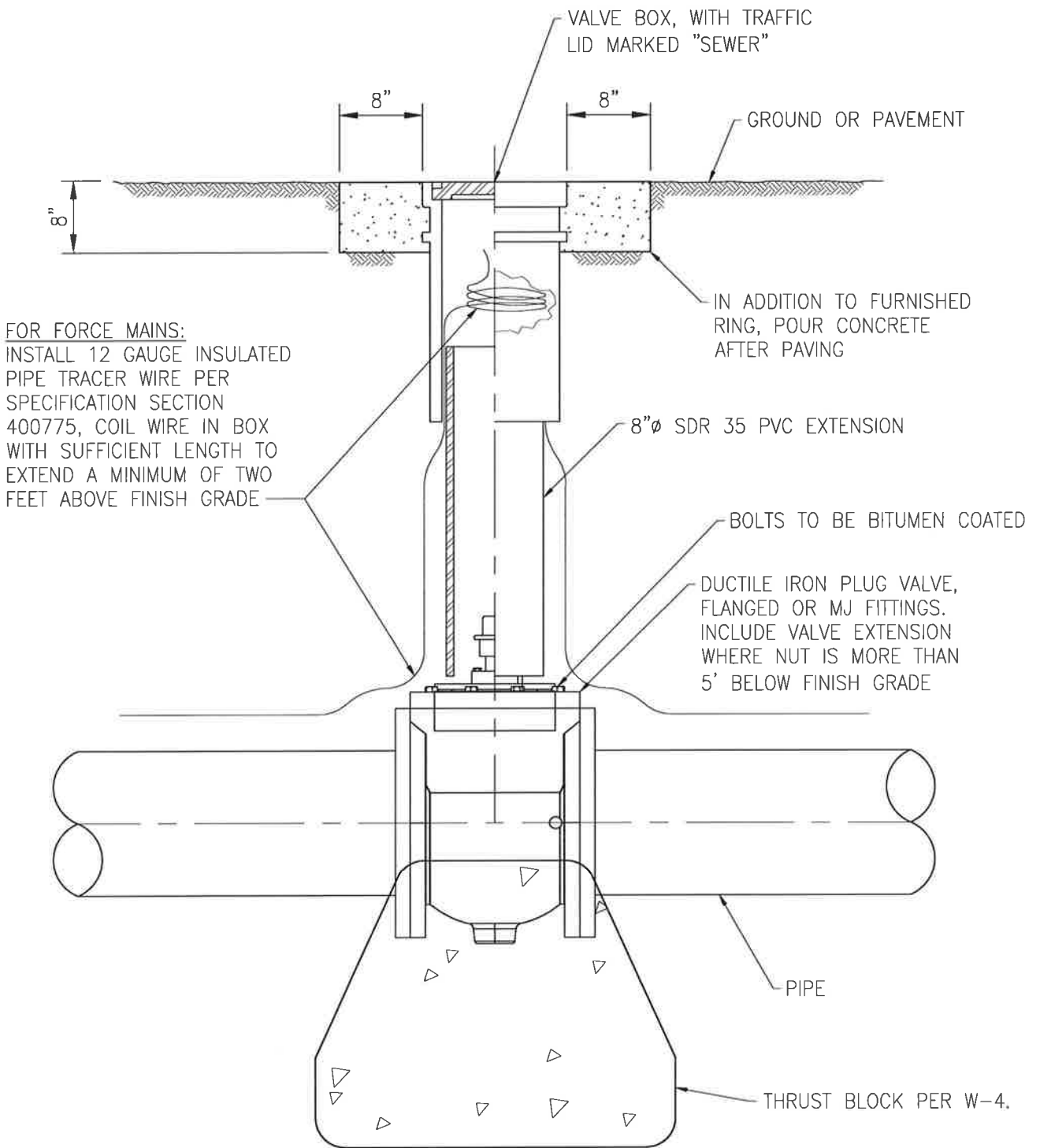
SECTION - ELEVATION
