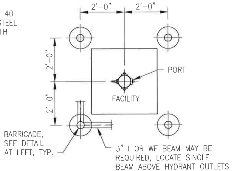
BOLLARD/BARRICADE PLAN
