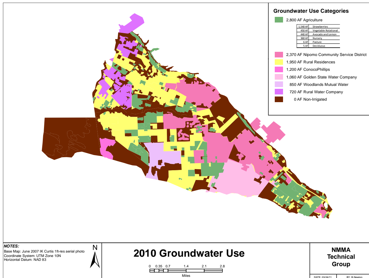
Figure 3-7. 2010 Groundwater Use
