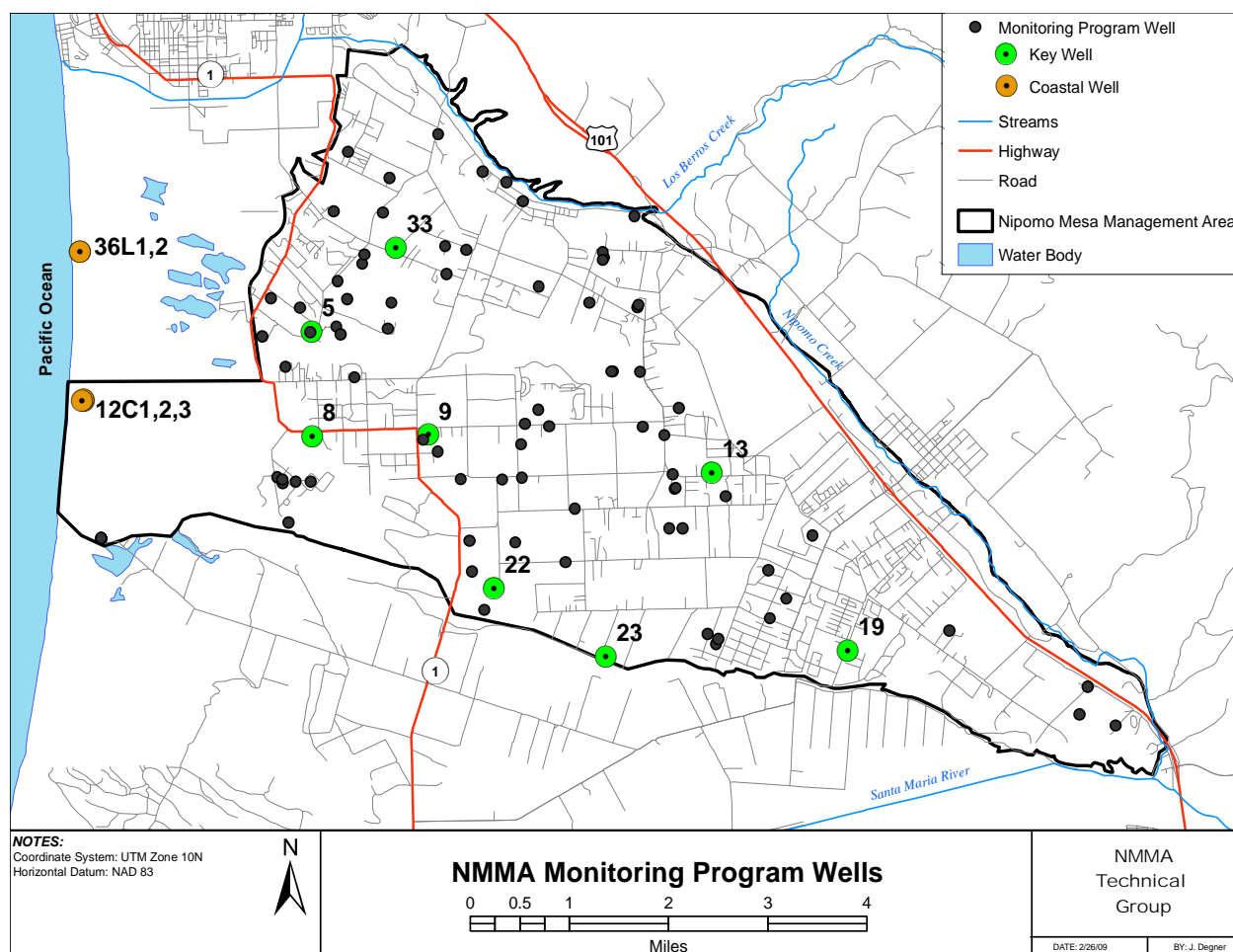
Figure 1-3. NMMA Monitoring Program Wells
