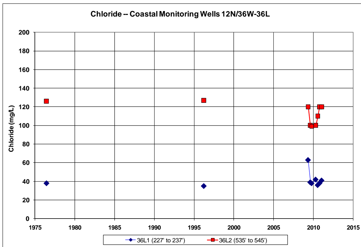
Figure 6-8. Chloride in Coastal Well 12N/36W-36L.
